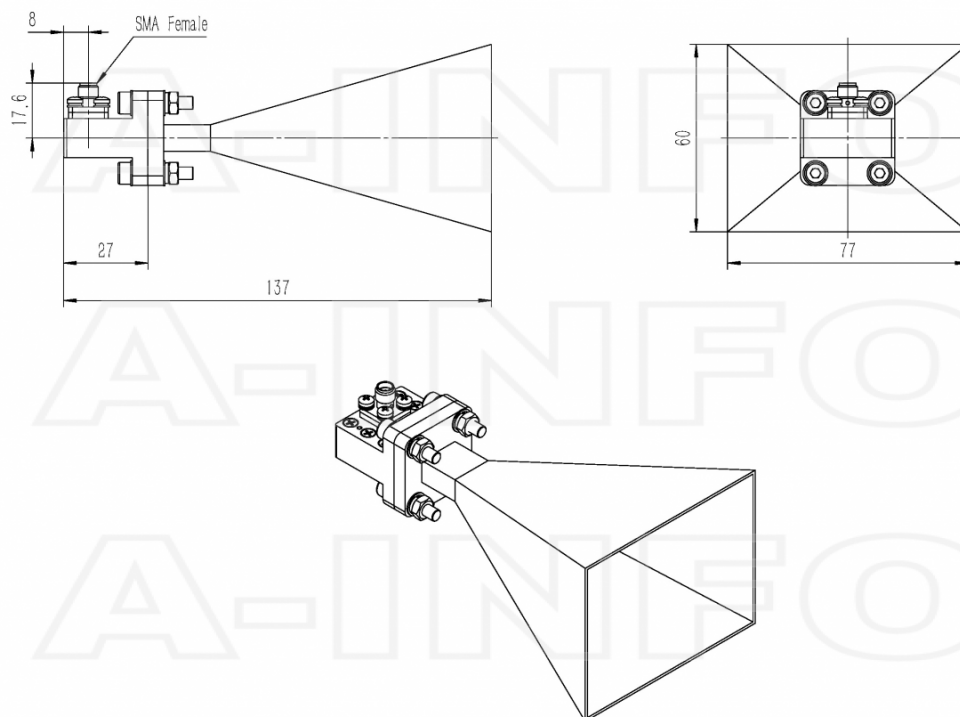
SMA-Female Output (P/N: LB-51-20-C-SF)
